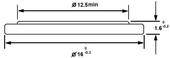
Dimensions are in millimetres
