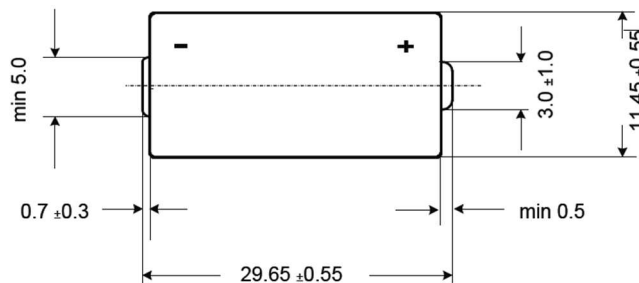
Dimensions are in millimeters and include label.
