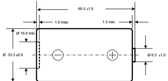
Dimensions are in millimeters and include label.
