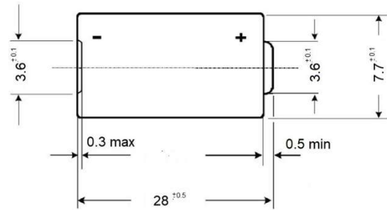
Dimensions are in millimeters and include label.
