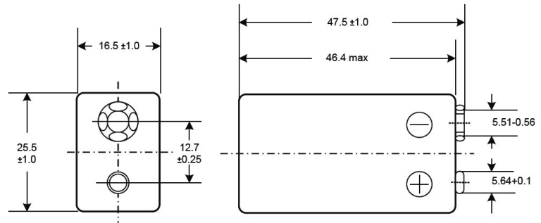
Dimensions are in millimeters and include label.
